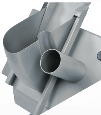
Filler neck for elongated material (dia. 59 mm)
